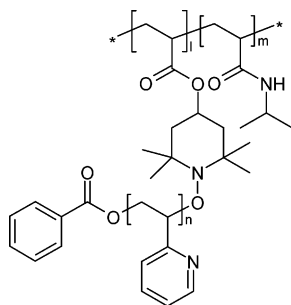
Scheme 1. Molecular Structure of Thermosensitive Copolymers
