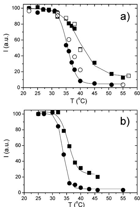
Figure 3. Normalized 1 H NMR signal intensities of -\text{CH}_3 groups in PNIPAM solution ( c_p = 5 \text{ mg/mL} , \text{pH} = 2 ) in dependence of temperature: (a) salt-free solution; (b) in 0.015 M NaCl. Solid symbols: heating; open symbols: cooling. ■, PNIPY-H; ●, PNIPY-L. Lines represent fits according to eq 6.
